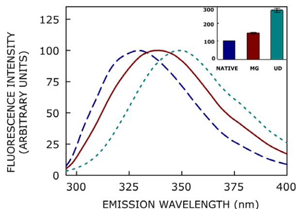
Fig. 2. Representative fluorescence emission spectra of BLA in native (blue, ---), molten globule (red, —) and urea-denatured (cyan, ---) states. The inset shows relative fluorescence intensities of BLA in native, molten globule (MG) and urea-denatured (UD) conformations at their respective emission maximum. The excitation wavelength was 280 nm in all cases. Spectra are intensity-normalized at the respective emission maximum. Data shown are means \pm SE of three independent measurements. All other conditions are as in Fig. 1. See Section 2 for other details. (For interpretation of the references to color in this figure legend, the reader is referred to the web version of this article.)
