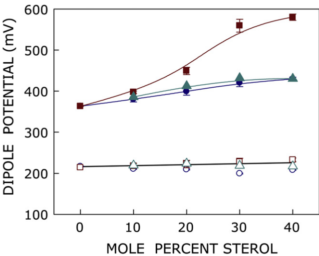
FIGURE 7 Invariance of dipole potential with sterol concentration in polyunsaturated (DAPC) membranes. Dipole potential in DAPC ( open symbols ) membranes is shown as a function of increasing concentrations of cholesterol ( \square ), 7-DHC ( \triangle ), and desmosterol ( \circ ). Dipole potential values in monounsaturated (POPC) membranes at the same sterol concentrations (cholesterol ( \blacksquare ), 7-DHC ( \blacktriangle ), and desmosterol ( \bullet )) are shown for comparison. Data points represent the mean \pm SE of at least three independent measurements. The ratio of di-8-ANEPPS to total lipid was 1:100 (mol/mol) and total lipid concentration was 0.43 mM. Measurements were carried out at room temperature ( \sim 23^{\circ}\text{C} ). Lines joining the data points merely serve as viewing guides. See Materials and Methods and the Supporting Material for details.
